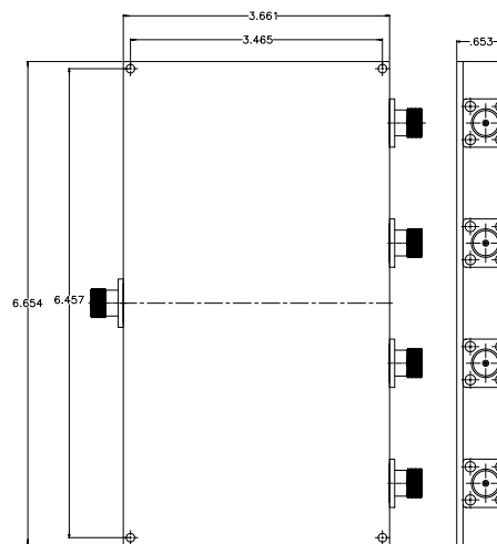
(300-500 MHz 4-Way Power Divider) (N)
