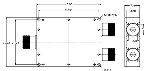
(300-500 MHz 2-Way Power Divider) (N)
