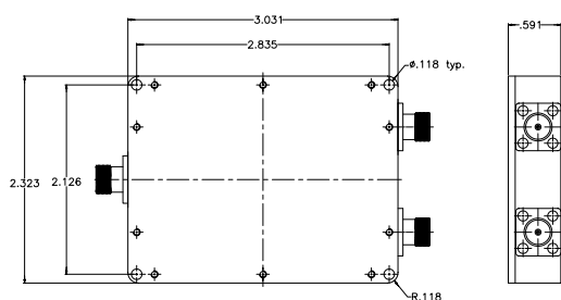
(300-500 MHz 2-Way Power Divider) (SMA)
