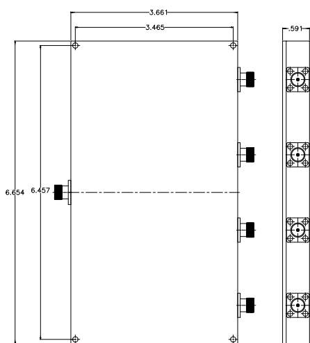
(300-500 MHz 4-Way Power Divider) (SMA)
