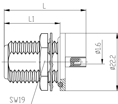
剥线尺寸 stripping dimensions
