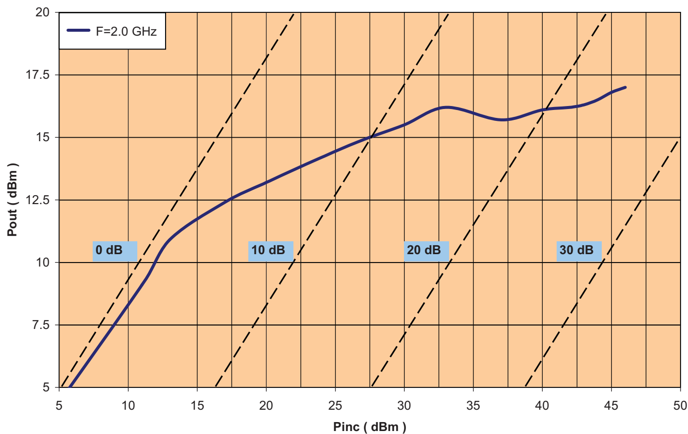
LM501202-M-C-300 Pout vs Pin Function ( C.W. )
