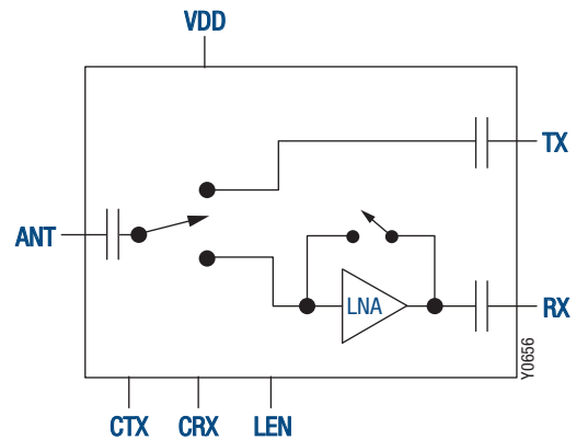
Figure 1. SKY85611-11 Block Diagram
