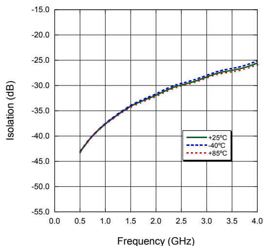
MASW-000825-12770T, RX Isolation Vs. Temperature Bias: +28V @ 0mA
