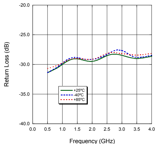
MASW-000825-12770T, RX Return Loss Vs. Temperature Bias: +5V @ 35mA
