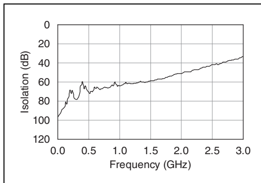
Figure 3. Typical Isolation
