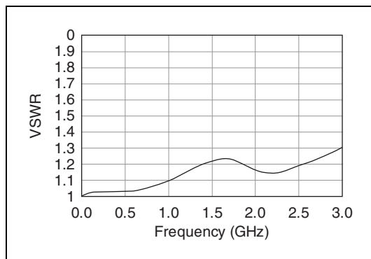
Figure 2. Typical VSWR
