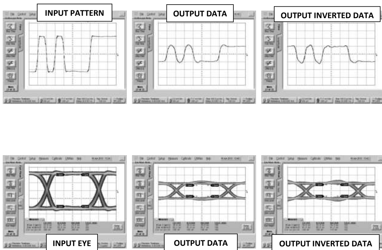
Fig. 6. Oscilloscope measurements of the BAL-0009SMG with a 10 Gb/s PRBS pattern. Bit pattern is measured with a 2^7-1 PRBS input demonstrating extremely good pulse fidelity for both inverted and non-inverted output. Eye diagrams are taken with a 2^{31}-1 PRBS input demonstrating minimal eye distortion/closure afforded by the extremely low frequency operation of the balun (<500 kHz).
