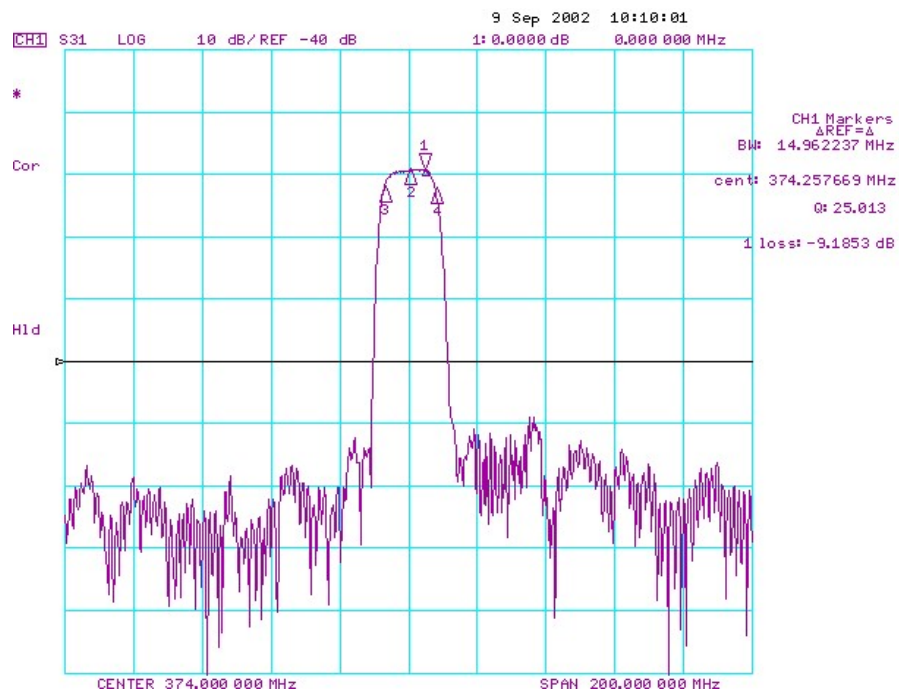
Fig-1 S21 Response Horizontal: 20MHz/Div
