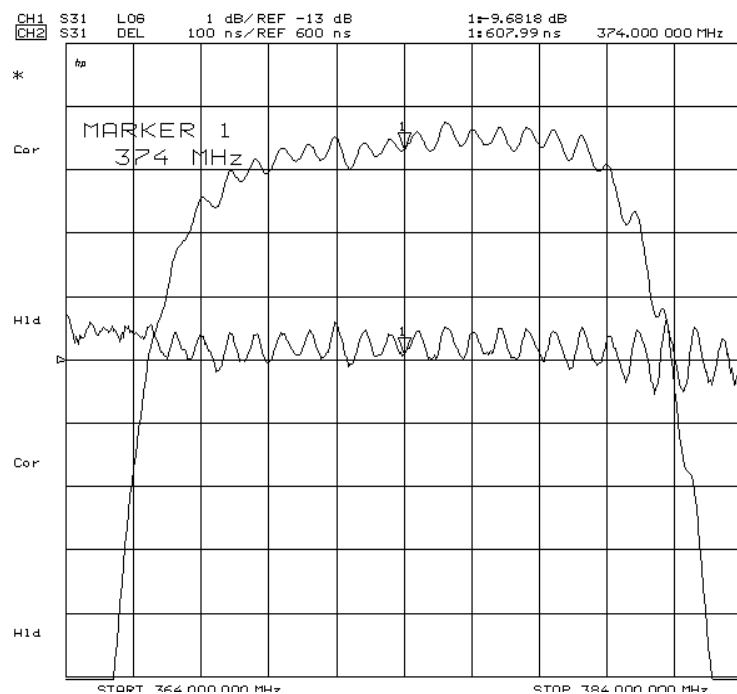
Fig-3 S21 Response Horizontal: 3 MHz/Div Vertical: 1dB/Div, Ref: -13dB
