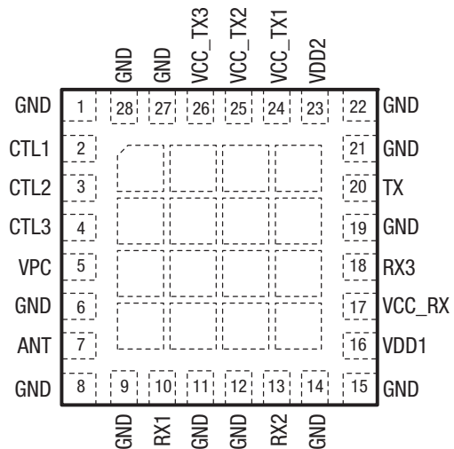
Figure 1. SKY65313-21 Pinout (Top View)
