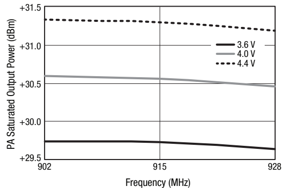
Figure 4. PA Saturated Output Power vs Frequency Over V_{CC\_TX1/2/3} ( V_{DD1} = V_{CC\_RX} = 3.3\text{ V} , T_c = 25\text{ }^{\circ}\text{C} , P_{IN} = +10\text{ dBm} , V_{PC} = 2.25\text{ V} )
