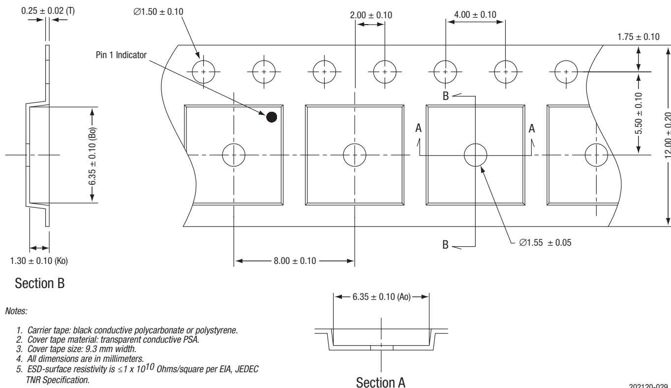
Figure 29. SKY65313-21 Tape and Reel Dimensions
