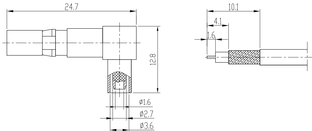
剥线尺寸 stripping dimension
