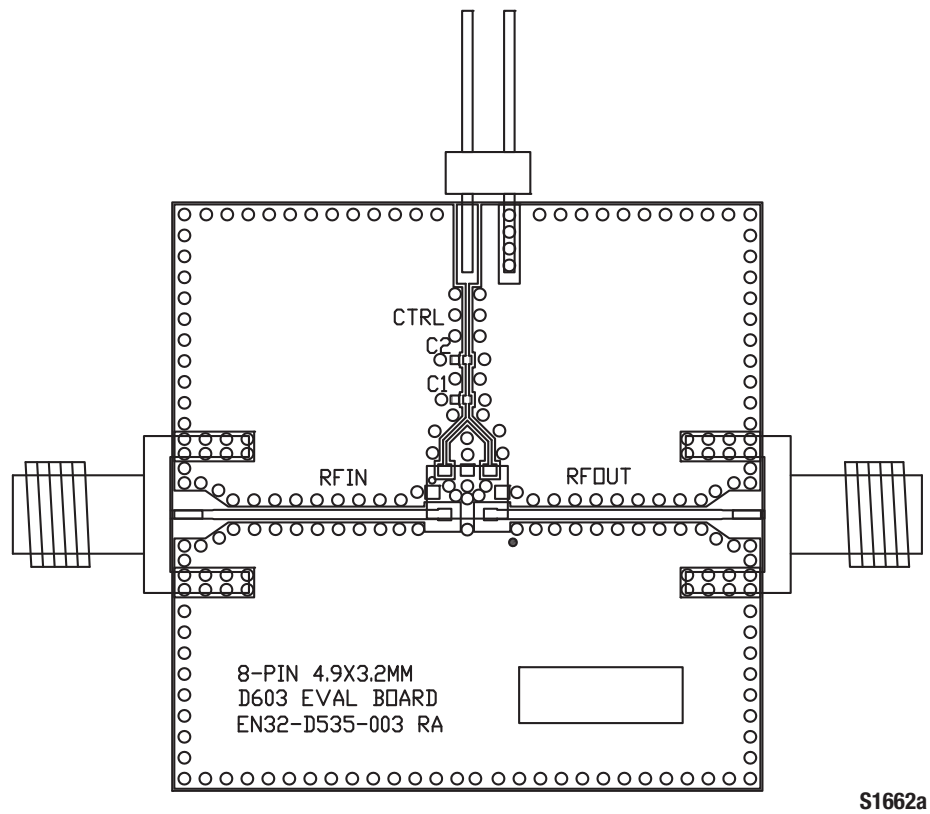
Figure 9. SKY12232-21 Evaluation Board Assembly Diagram
