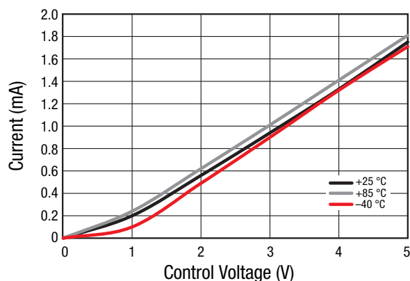
Figure 6. Current vs Control Voltage Over Temperature
