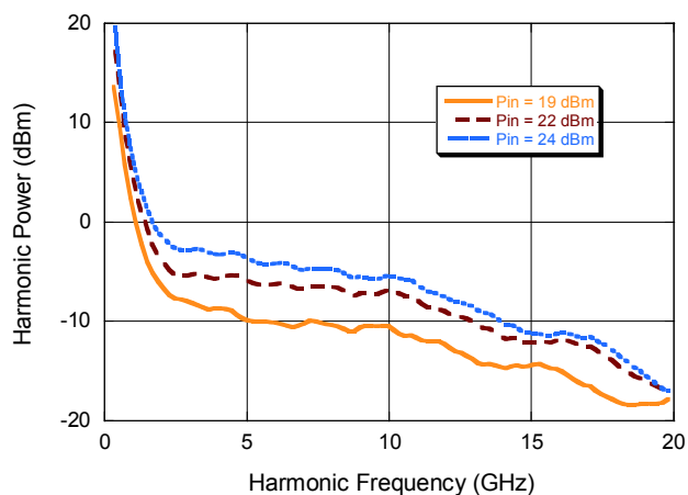
Harmonic Output, 300 MHz Input Frequency
