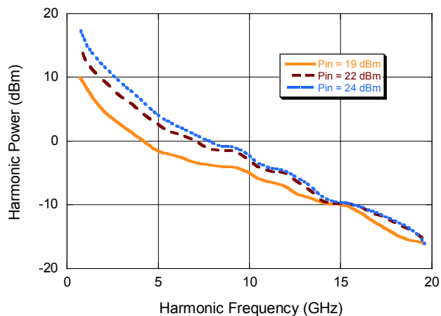
Harmonic Output, 700 MHz Input Frequency
