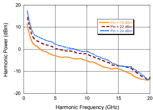
Harmonic Output, 500 MHz Input Frequency
