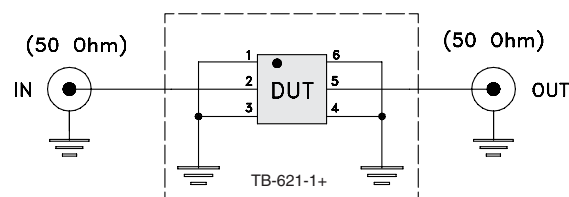
Fig 1. Block diagram of Test Circuit used for characterization, Test board TB-621-1+ Conditions: Attenuation, VSWR: Pin=-10 dBm
