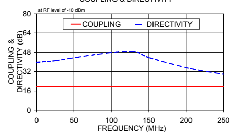
PDC-20-3+ COUPLING & DIRECTIVITY
