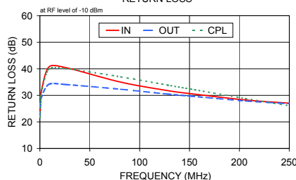
PDC-20-3+ RETURN LOSS
