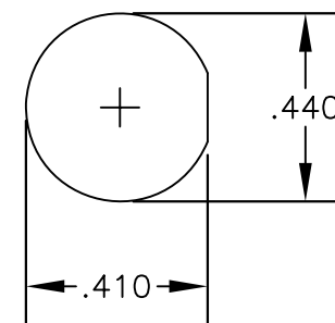
MOUNTING HOLE
