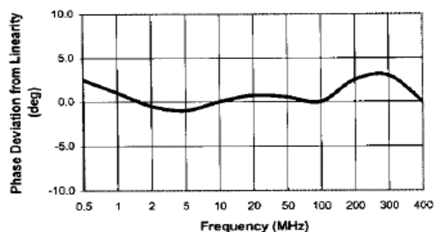
Phase Linearity
