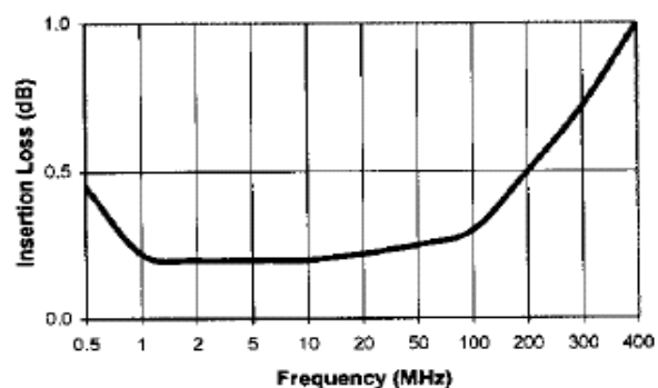
Insertion Loss
