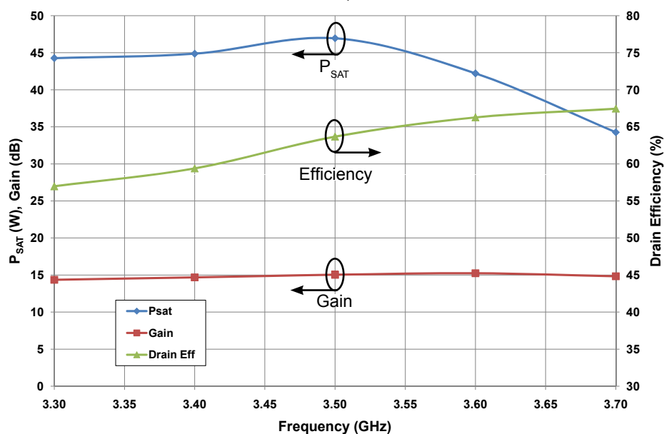
P_{SAT} Gain, and Drain Efficiency vs Frequency of the CGH40035F in the CGH40035F-AMP
