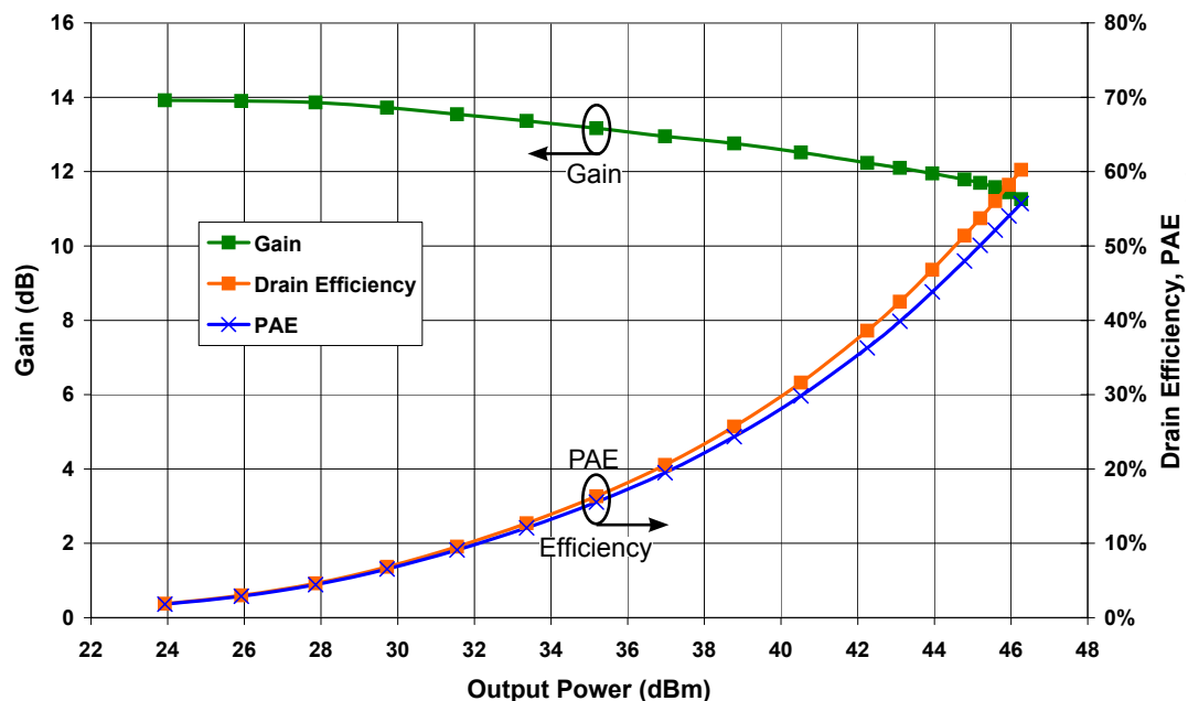
Swept CW Data of CGH40035 vs. Output Power with Source and Load Impedances Optimized for P_{SAT} Power in CGH40035F-AMP V_{DD} = 28\text{ V} , I_{DQ} = 500\text{ mA} , Freq = 3.5 GHz
