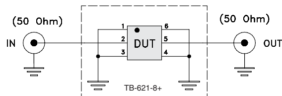
Fig 1. Block diagram of Test Circuit used for characterization, Test board TB-621-8+ Conditions: Attenuation, VSWR: Pin=-10 dBm
