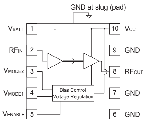
Figure 1: Block Diagram
