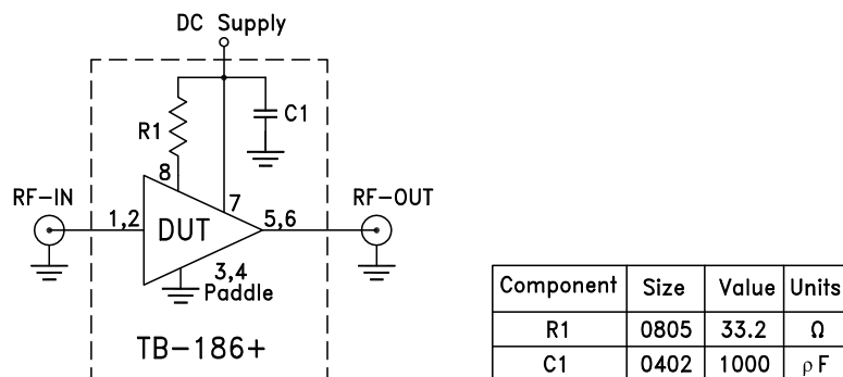
Fig 1. Block Diagram of Test Circuit used for characterization. (DUT soldered on Mini-Circuits Characterization test board TB-313)
