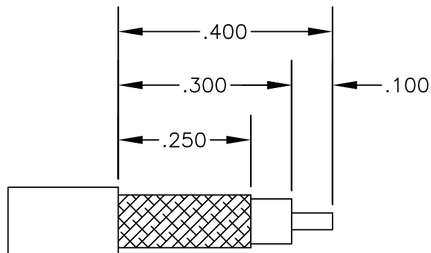
STRIPPING DIMENSIONS
