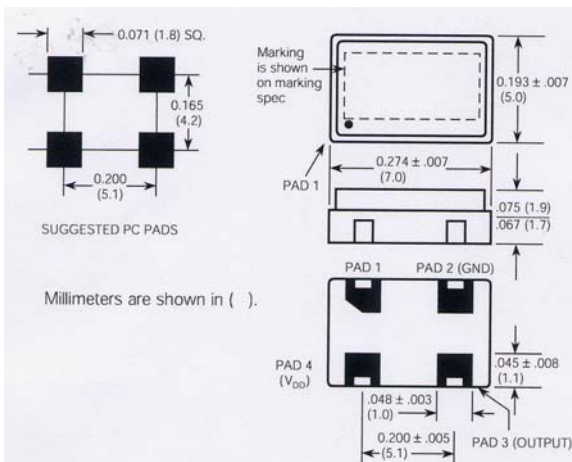
Fig. 2. "T" Package
