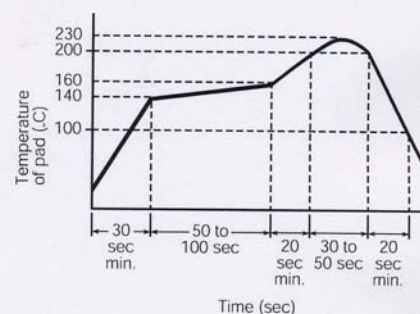
Fig. 1. Recommended Reflow Soldering Profile
