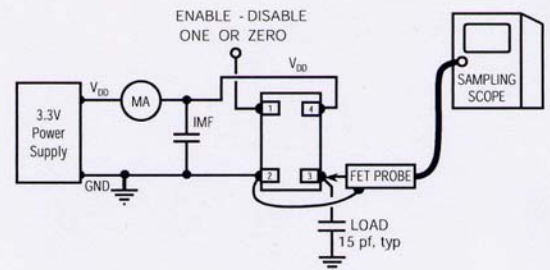
Fig. 4. Test Circuit
