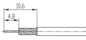
剥线尺寸 stripping dimension
