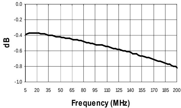
Insertion Loss 1
