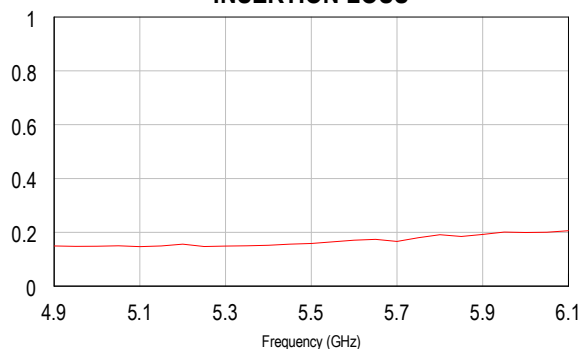
INSERTION LOSS
