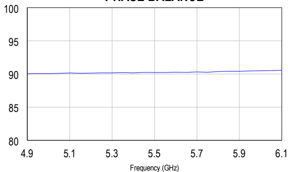
PHASE BALANCE
