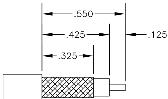
STRIPPING DIMENSIONS
