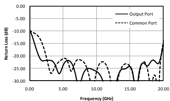
Fig. 2. Return loss for output and common ports.
