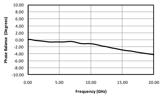
Fig. 4. Phase balance between output ports.
