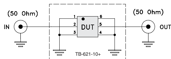
Fig 1. Block diagram of Test Circuit used for characterization, Test board TB-621-10+ Conditions: Attenuation, VSWR: Pin=-10 dBm
