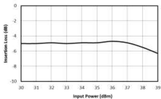
Fig. 6. Output Compression
