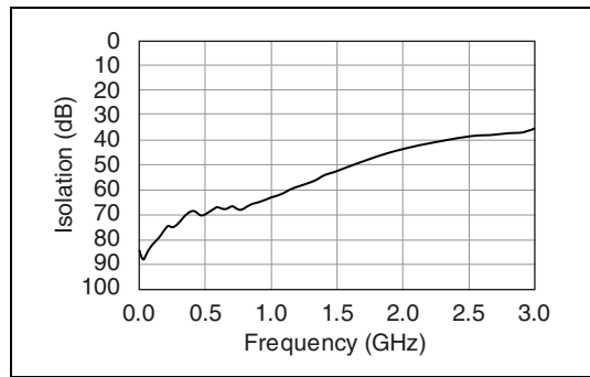
Figure 3. Typical Isolation
