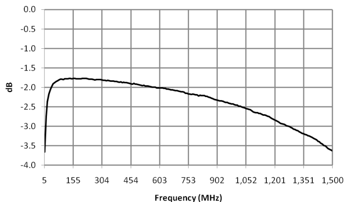
MABA-011015 insertion_loss_2_pin1_3
