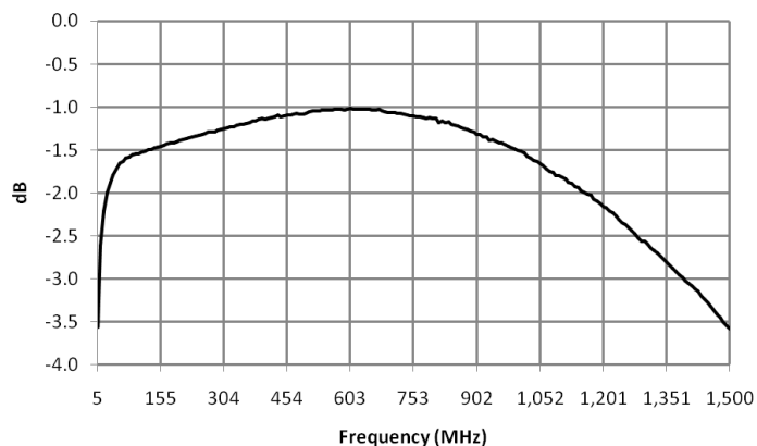
MABA-011015 insertion_loss_1_pin1_5
