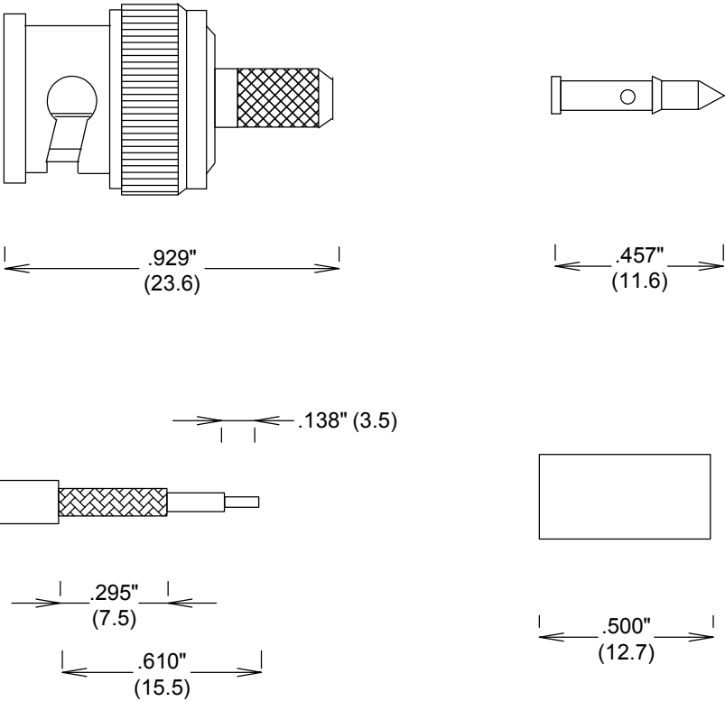
STRIPPING DIMENSIONS
