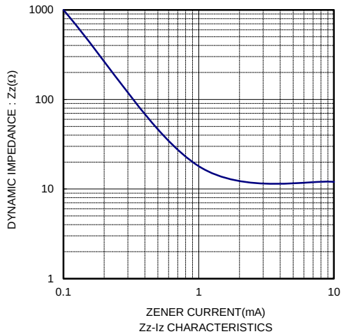
Z_z - I_z CHARACTERISTICS
