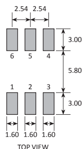
SOLDER PAD LAYOUT
