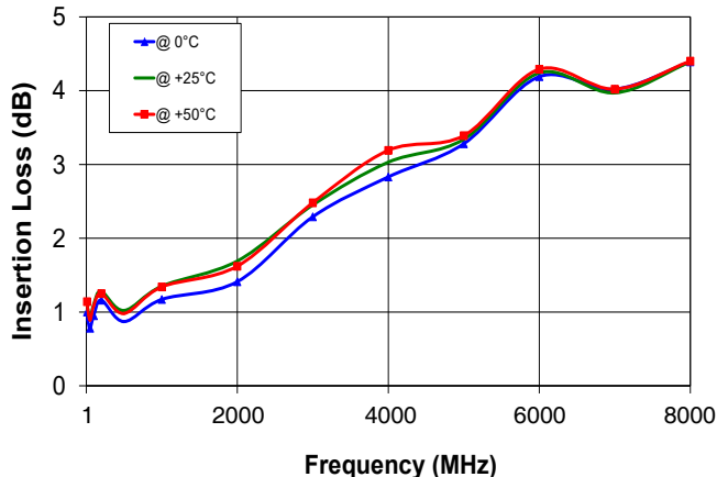
Insertion Loss @ Input Power +28 dBm vs. Frequency over Temperatures
