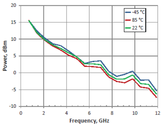
Harmonic Output, 22 dBm Input Power
