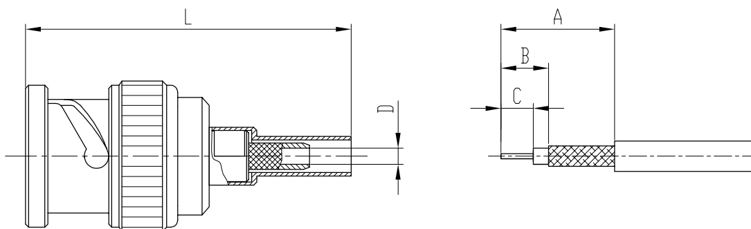
剥线尺寸 stripping dimensions
