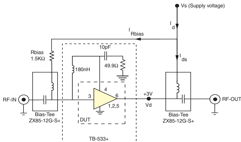
Fig 1. Block Diagram of Test Circuit used for characterization. (DUT soldered on Mini-Circuits Characterization Test Board TB-533+) Gain, Output power at 1dB compression ( P_{1dB} ), output IP3 (OIP3) and Noise Figure measured using Agilent's N5242A PNA-X microwave network analyzer.
