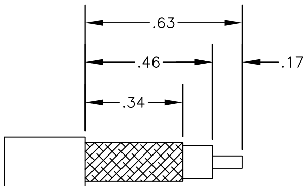
STRIPPING DIMENSIONS
