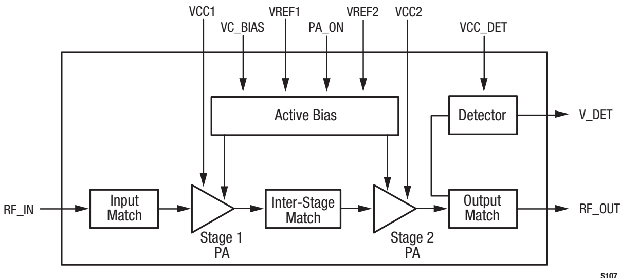
Figure 2. SKY65131 Block Diagram
