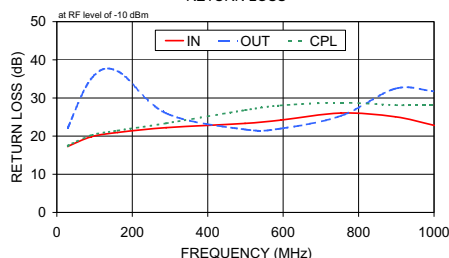
LRDC-10-2-75J RETURN LOSS
