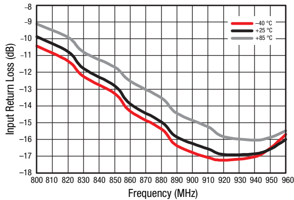
Figure 18. Small Signal Input Return Loss (IS11I) vs Frequency and Temperature, Narrow Band
