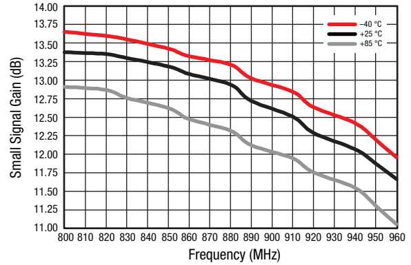
Figure 17. Small Signal Gain (IS21I) vs Frequency and Temperature, Narrow Band
