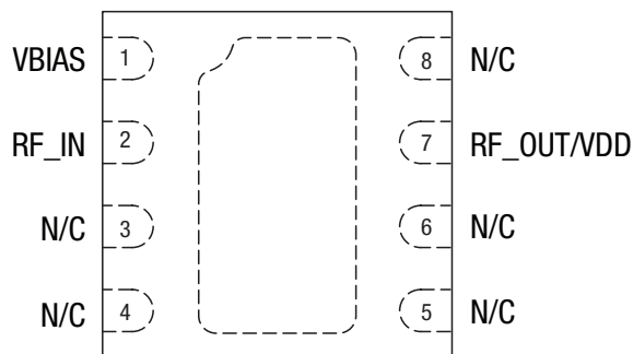
Figure 2. SKY67013-396LF Pinout – 8-Pin DFN (Top View)
