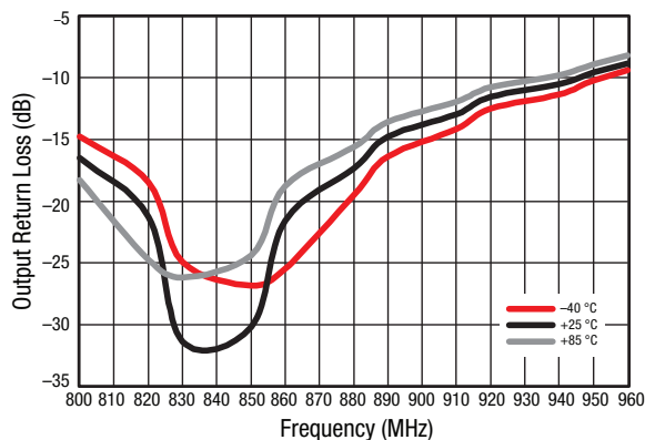
Figure 20. Small Signal Output Return Loss (S22) vs Frequency and Temperature, Narrow Band
