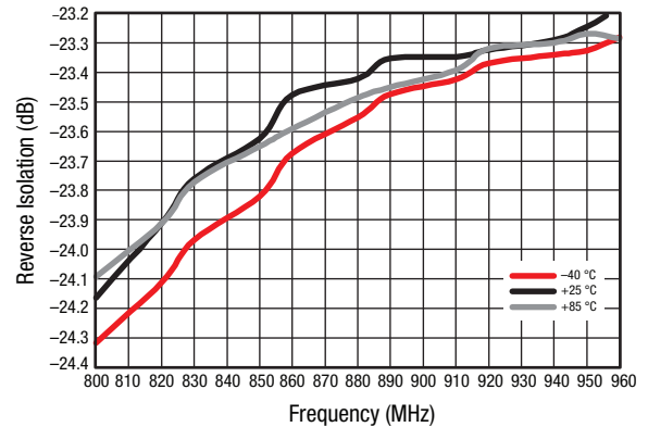
Figure 19. Small Signal Reverse Isolation (IS12I) vs Frequency and Temperature, Narrow Band
