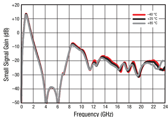
Figure 21. Small Signal Gain (S21) vs Frequency and Temperature, Wide Band
