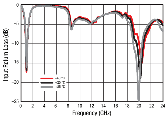
Figure 22. Small Signal Input Return Loss (S11) vs Frequency and Temperature, Wide Band
