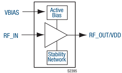
Figure 1. SKY67013-396LF Block Diagram
