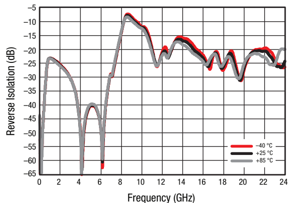
Figure 23. Small Signal Reverse Isolation (S12) vs Frequency and Temperature, Wide Band
