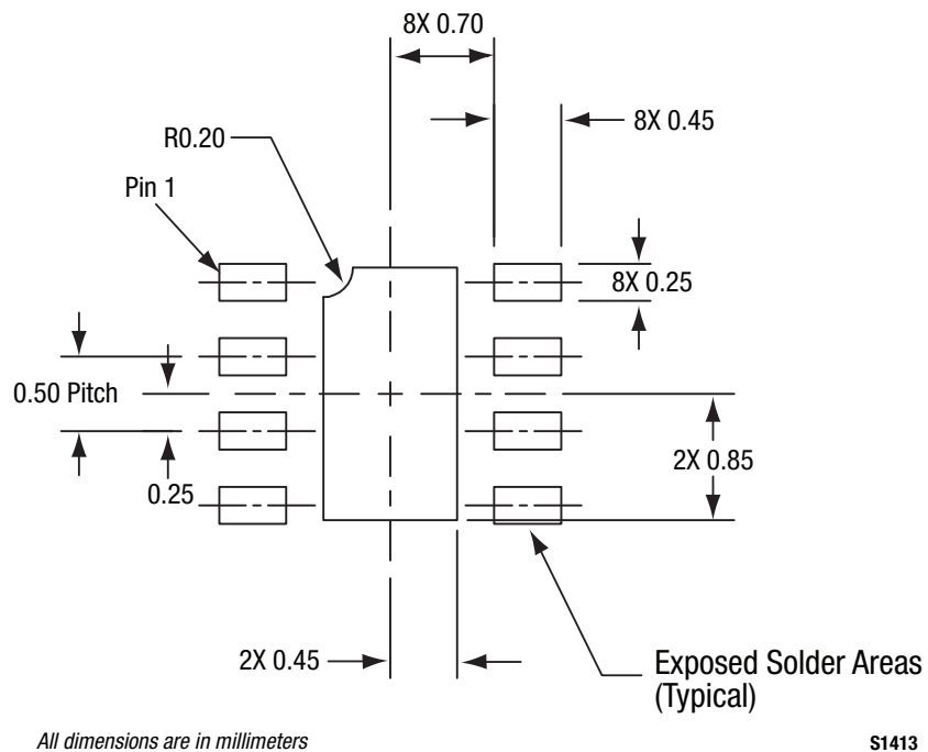
Figure 29. SKY67013-396LF PCB Layout Footprint (Top View)
