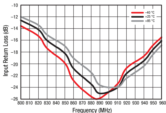
Figure 5. Small Signal Input Return Loss (IS11I) vs Frequency and Temperature, Narrow Band
