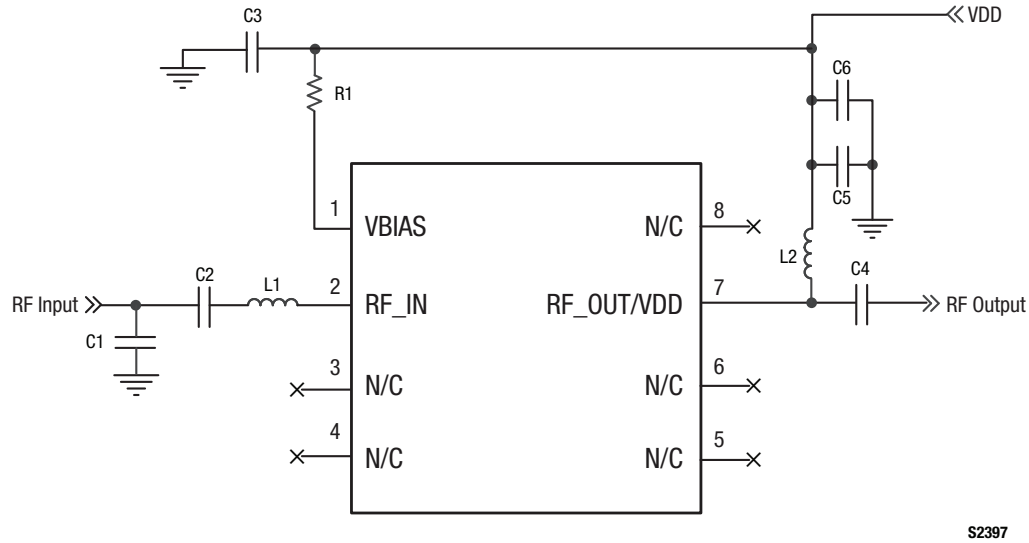
Figure 28. SKY67013-396LF Evaluation Board Schematic
