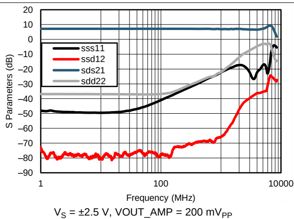
Figure 9. S-Parameters ( \pm 2.5\text{-V} Supply)
