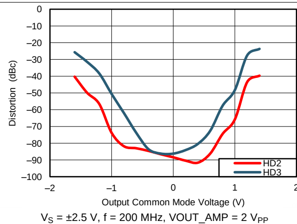
Figure 18. HD2 and HD3 vs Output Common-Mode Voltage
