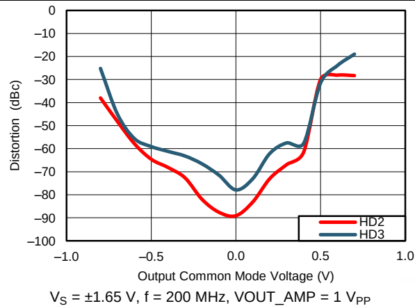
Figure 19. HD2 and HD3 vs Output Common-Mode Voltage
