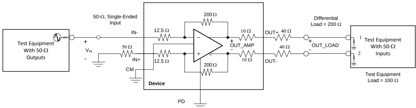
Figure 49. Test Schematic: Single-Ended Input, Differential Output
