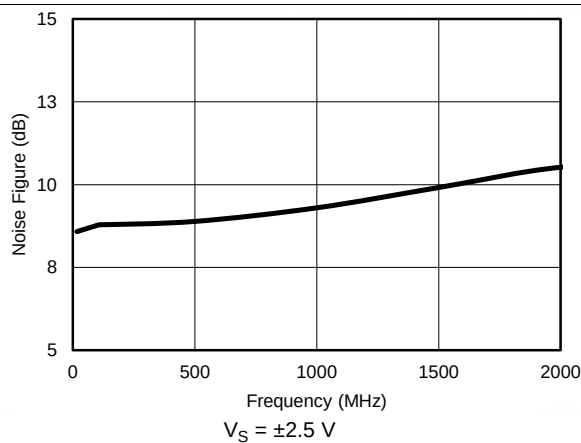
Figure 35. Noise Figure vs Frequency
