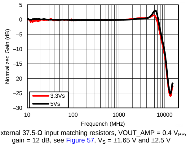
Figure 2. Frequency Response Differential Input
