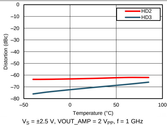
Figure 15. HD2 and HD3 vs Temperature
