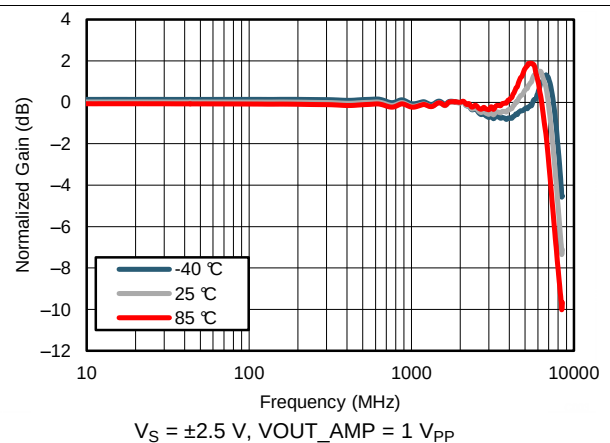
Figure 6. Frequency Response vs Temperature
