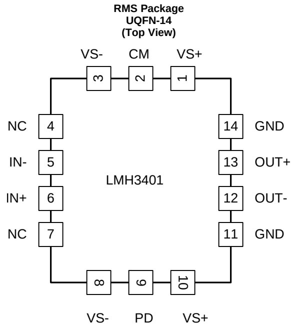
Pin Functions
