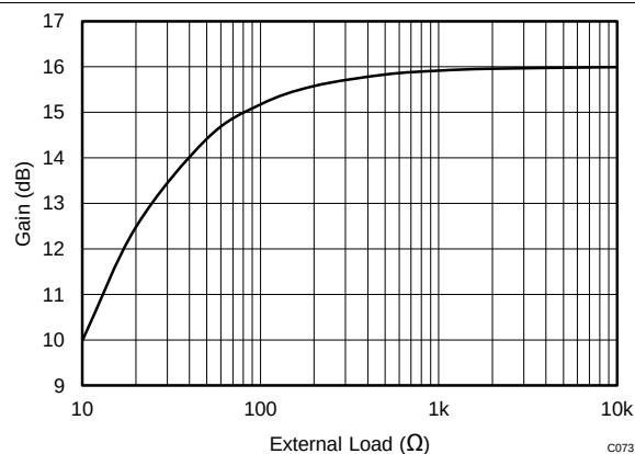
Figure 70. Net Gain versus Load Resistance
