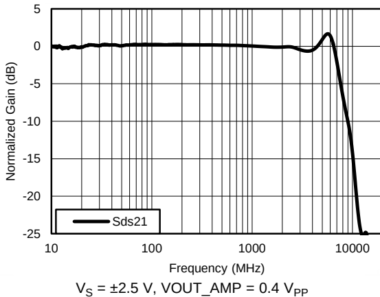
Figure 1. Frequency Response Single-Ended Input
