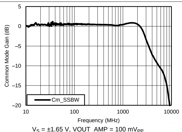
Figure 12. Common-Mode Frequency Response
