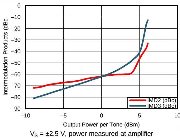
Figure 33. Intermodulation Distortion (f = 1000 MHz)
