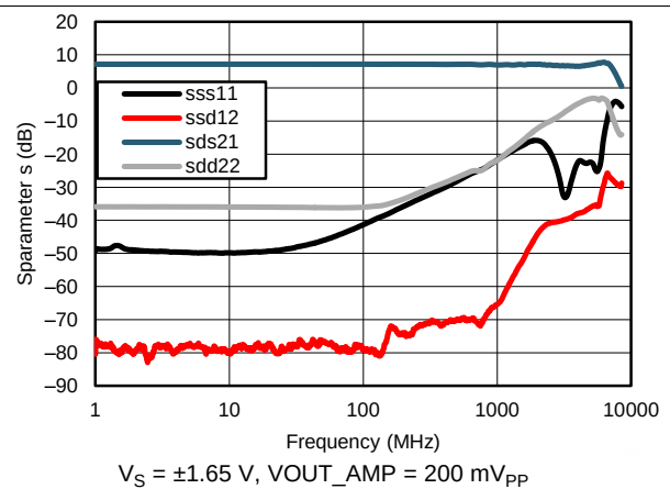
Figure 10. S-Parameters (3.3-V Supply)
