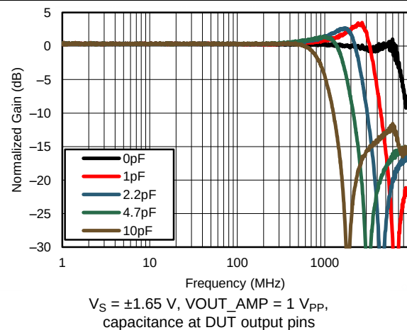
Figure 8. Frequency Response with Capacitive Load
