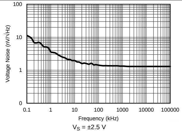
Figure 34. Input-Referred Voltage Noise
