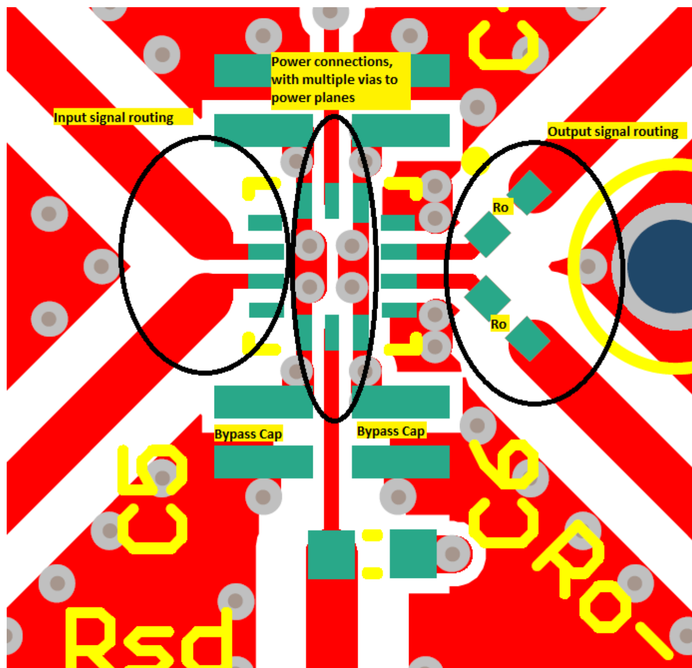
Figure 71. Layout Example
