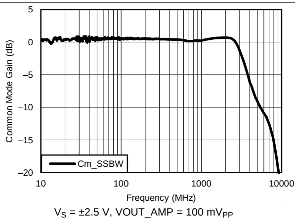
Figure 11. Common-Mode Frequency Response
