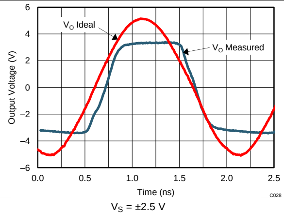
Figure 44. Overdrive Recovery
