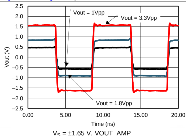
Figure 38. Pulse Response for Various V_O
