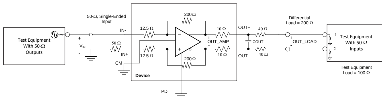
Figure 52. Test Schematic for Capacitive Load
