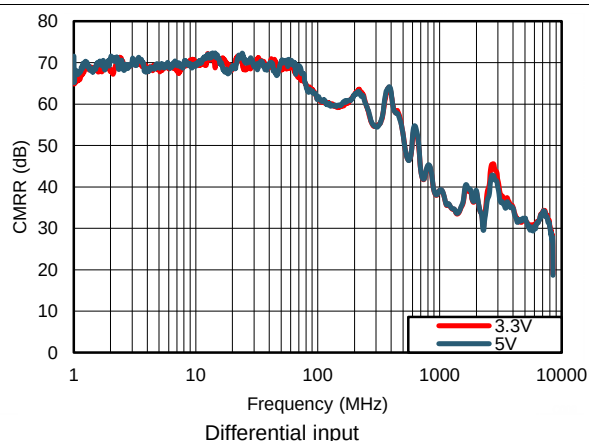
Figure 40. CMRR (Sdc21)
