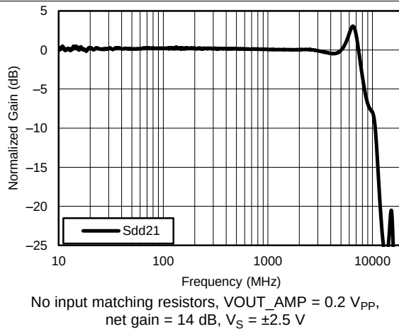
Figure 3. Frequency Response Differential Input
