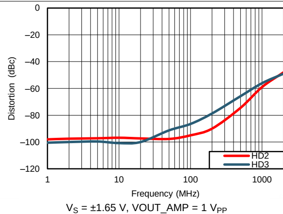
Figure 16. HD2 and HD3 ( 3.3\text{-V } V_S )
