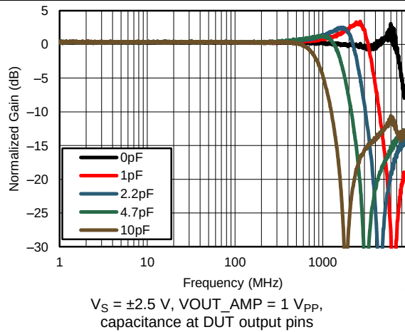
Figure 7. Frequency Response with Capacitive Load
