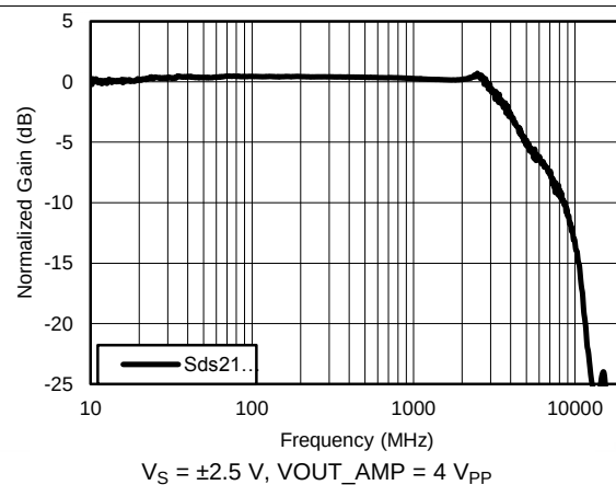
Figure 5. Large-Signal Frequency Response (Single-Ended Input)
