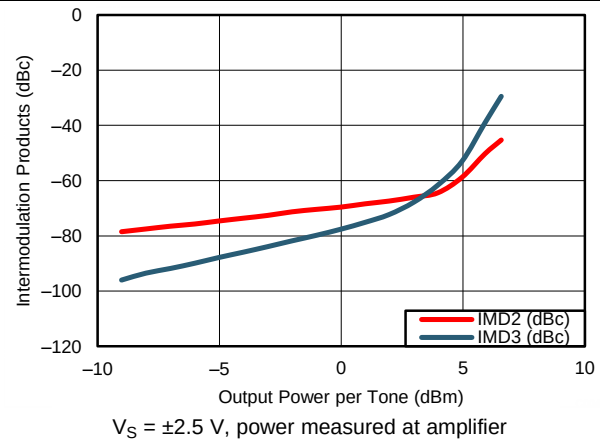
Figure 32. Intermodulation Distortion (f = 500 MHz)
