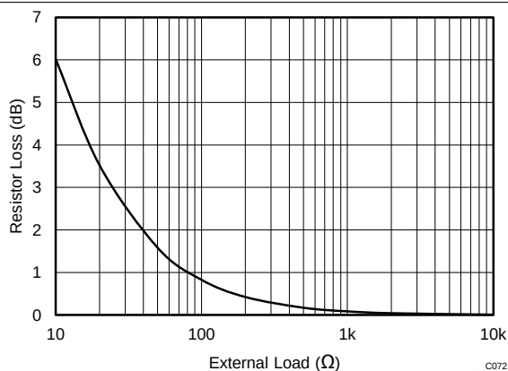
Figure 69. Gain Loss Due to On Chip Output Resistors
