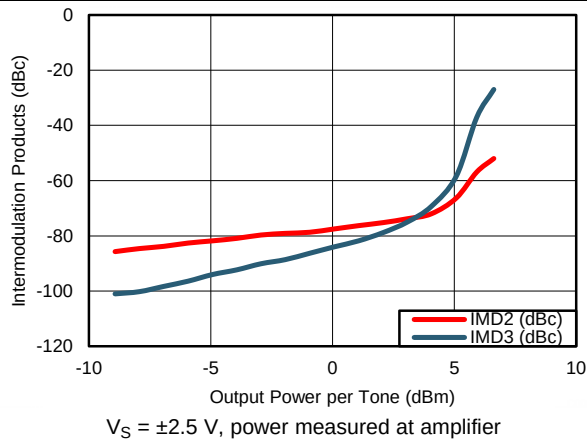
Figure 31. Intermodulation Distortion (f = 200 MHz)
