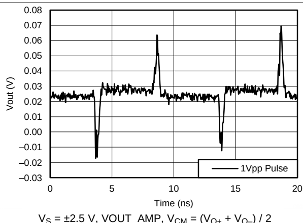
Figure 37. Pulse Response Common-Mode
