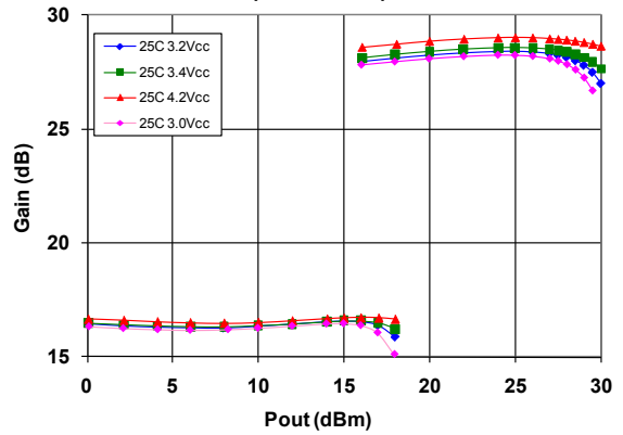
Figure 4: WCDMA Gain (dB) over Voltage ( T_c = 25 °C)
