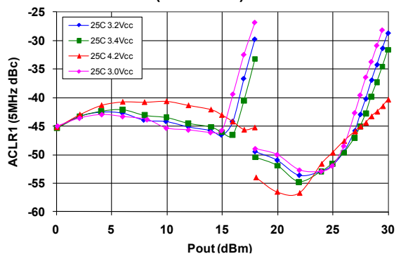
Figure 8: WCDMA ACLR1 (dBc) over Voltage ( T_c = 25 °C)
