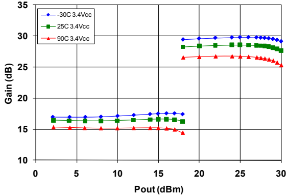
Figure 3: WCDMA Gain (dB) over Temperature ( V_{BATT} = V_{CC} = 3.4 V)
