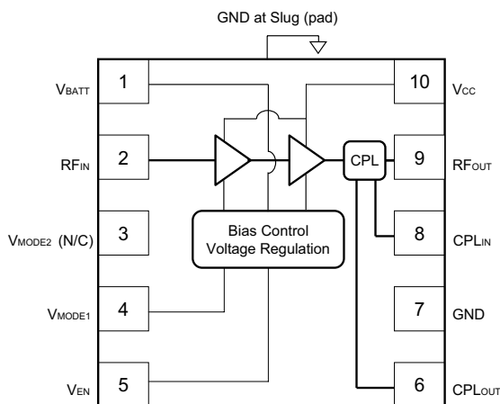
Figure 1: Block Diagram
