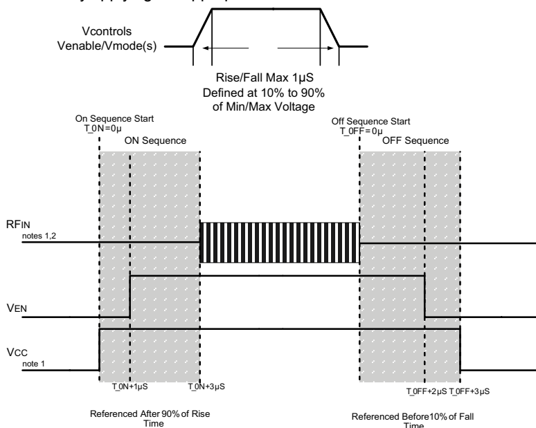
Figure 9: Recommended ON/OFF Timing Sequence
