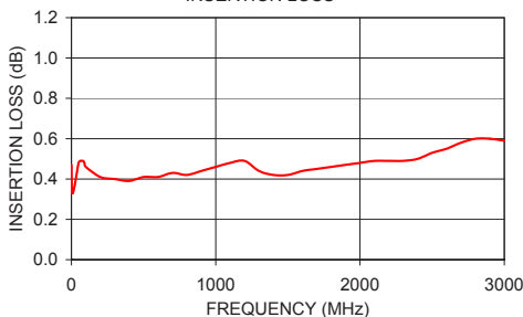
ZFBT-33W-75-FT+ INSERTION LOSS
