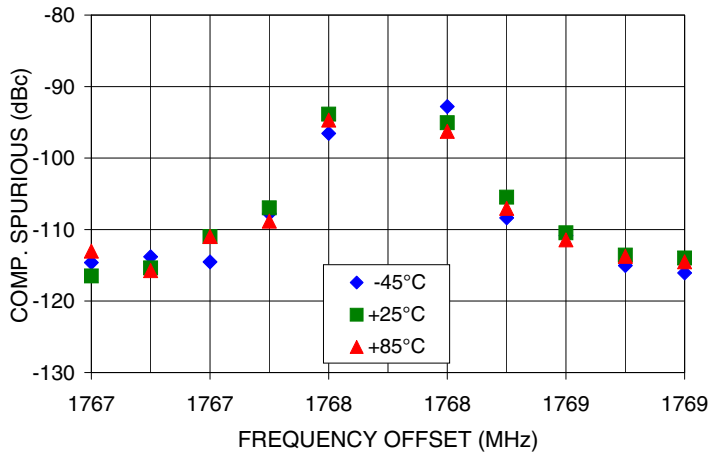
COMPARISON SPURIOUS Vs FREQ. OFFSET @ Fcar = 1768MHz
