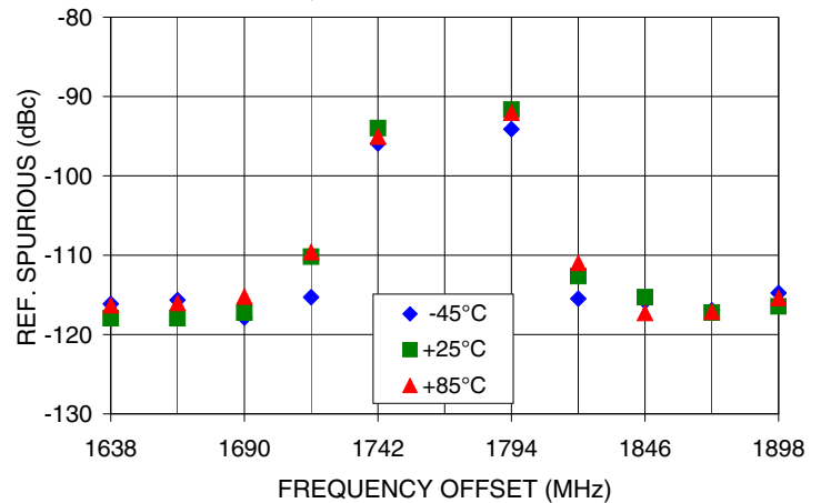
REFERENCE SPURIOUS Vs FREQ. OFFSET @ Fcar = 1768MHz
