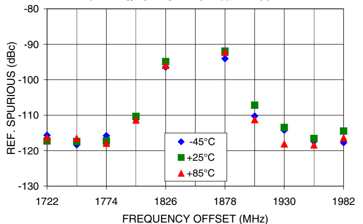
REFERENCE SPURIOUS Vs FREQ. OFFSET @ Fcar = 1852MHz
