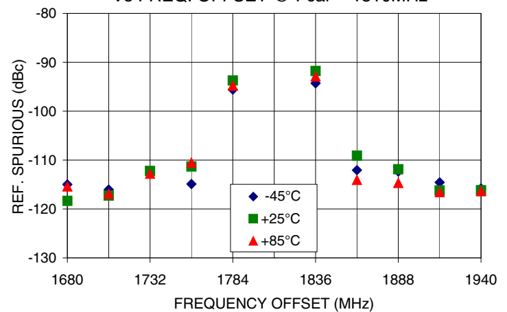
REFERENCE SPURIOUS Vs FREQ. OFFSET @ Fcar = 1810MHz
