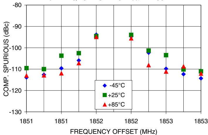
COMPARISON SPURIOUS Vs FREQ. OFFSET @ Fcar = 1852MHz
