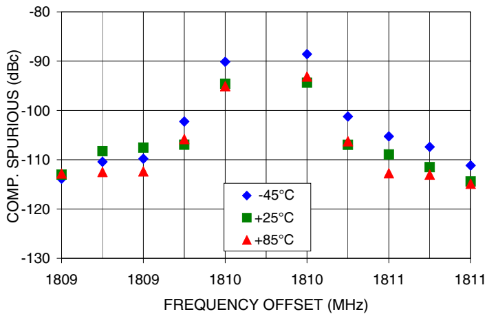
COMPARISON SPURIOUS Vs FREQ. OFFSET @ Fcar = 1810MHz
