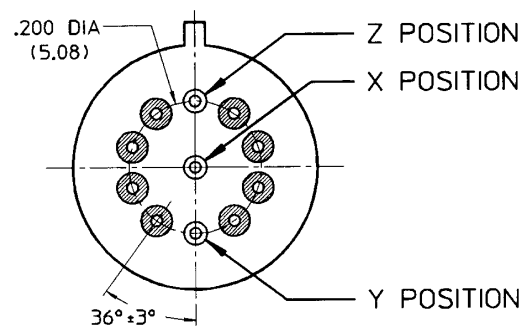
Figure 3. Ground Pin Positions.
