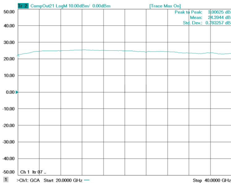
Figure 1-1: ERZ-LNA-2000-4000-24 Psat
