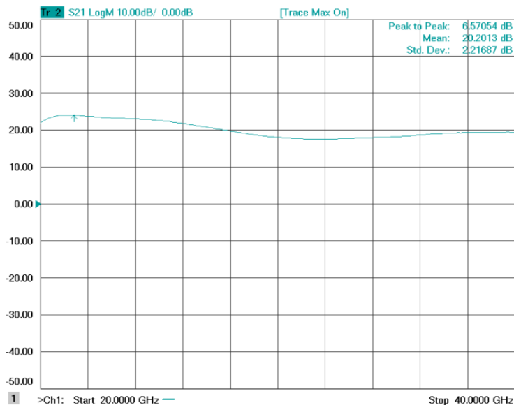
Figure 1-2: ERZ-LNA-2000-4000-24 Small Signal Gain
