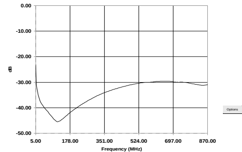
Coupled Port Return Loss
