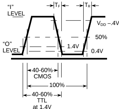
WAVEFORMS
